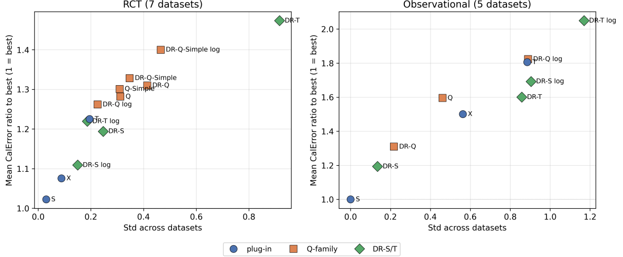
Figure 2: Mean calibration-error ratio to the best-calibrated learner per dataset (1 = best) vs. cross-dataset standard deviation of the ratio, for RCT (left) and observational (right) datasets. Each learner at its best calibration configuration. The ideal learner sits at the bottom-left corner (low ratio, low variance).
