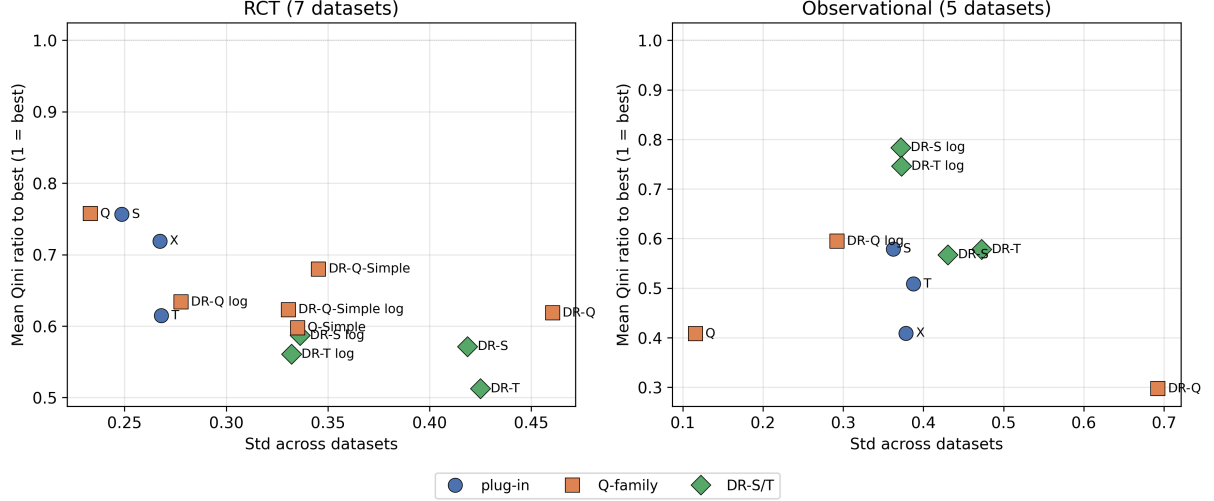
Figure 1: Mean Qini ratio to the best learner per dataset ( 1 = \text{best} ) vs. cross-dataset standard deviation of the ratio, for RCT (left) and observational (right) datasets. The ideal learner sits in the upper-left corner (high ratio, low variance).
